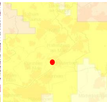
Abb. 21: NO 2 -Belastung
